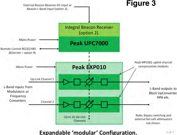
Expandable 'modular' Configuration.
