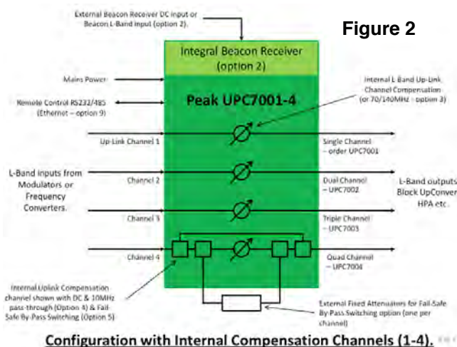
Configuration with Internal Compensation Channels (1-4).
